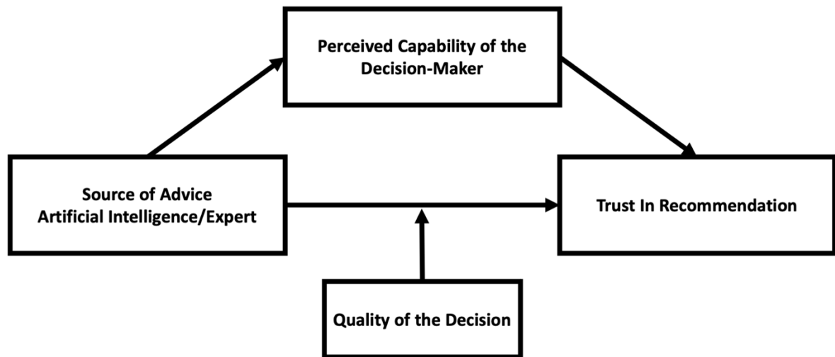
Figure 1 Theoretical Model
