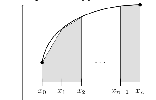
Trapezoidal approximation
