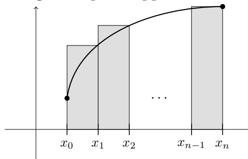
Right-endpoint approximation
