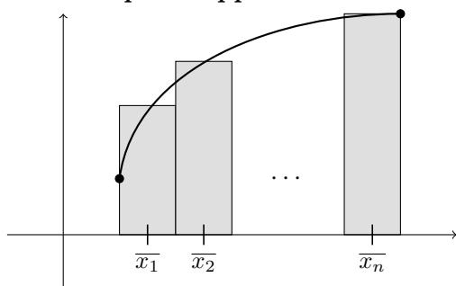
Midpoint approximation
