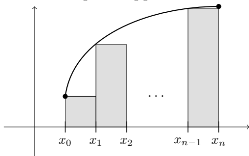
Left-endpoint approximation
