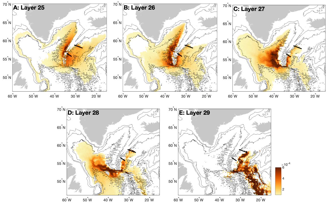
Figure 7: Probability distributions of 10-year simulated particle trajectories after initialization at two locations ( \sim 58^\circ\text{N} and \sim 56^\circ\text{N} ) along the eastern flank of the Reykjanes Ridge in A) layer 25, B) layer 26, C) layer 27, D) layer 28 and E) Layer 29. Black lines indicate particle release sites. Bathymetry is contoured every 1000 meters.
