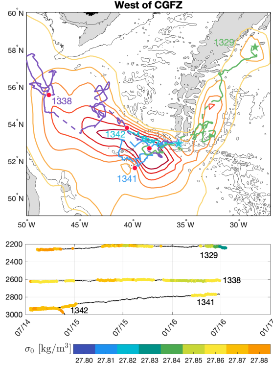
Figure 12: Same as Figure 9 except particle distribution maps are for layer 28 and RAFOS float trajectories occupy a density range of, approximately, between 27.86 - 27.88 \text{ kg m}^{-3} .
