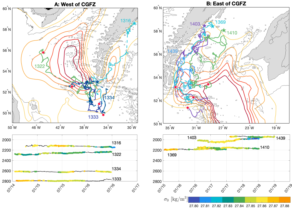
Figure 11: Same as Figure 9 except particle distribution maps are for layer 27 and RAFOS float trajectories occupy a density range of, approximately, between 27.84 - 27.86 kg m -3 .
