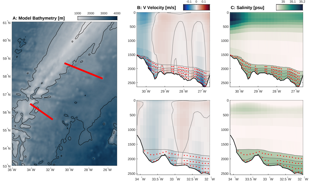
Figure 2: Particle release locations and depths. A) Locations where particles are released from are indicated in red and overlaid on model bathymetry. B) Cross section of mean (1978 - 2022) meridional velocity and, C) salinity, from north (top) and south (bottom) release locations. Black lines represent isopycnals of the ISOW layer and red dots indicate location and depths where particles are released. Gray contours indicate the time mean model isotach. Particles are released where the time average flow is southward.
