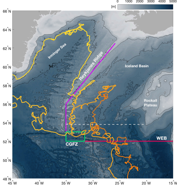
Figure 3: Reykjanes Ridge (purple) and WEB (red/pink) gates along with CGFZ box (green) used to classify particle exit pathways from the Iceland Basin. Overlaid are examples of particle trajectories (yellow/orange). Bathymetry is plotted in the background and contoured every 1000 meters. Dashed gray line identifies the section across which monthly volume transports are calculated in section 3.1.
