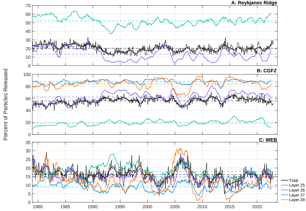
Figure 4: Percent of simulated particles released to exit the Iceland Basin, A) over the Reykjanes Ridge, B) through the Charlie Gibbs Fracture Zone or C) southward into the WEB. Colors indicate the isopycnal layer the particles were released within, where turquoise = layer 25, purple = layer 26, blue = layer 27 and orange/red = layer 28. Black represents the sum total over all the layers. Dashed lines indicate the time averaged percentage of particles to exit via each pathway. Time series are smoothed using a 12-month boxcar moving mean filter. In panel A, only particles from layers 25 and 26 crossed the ridge while deeper particles were blocked by the bathymetry. Note the sum totals in each panel (black) do not perfectly add up to 100% because a small number of particles stay within the Iceland Basin.
