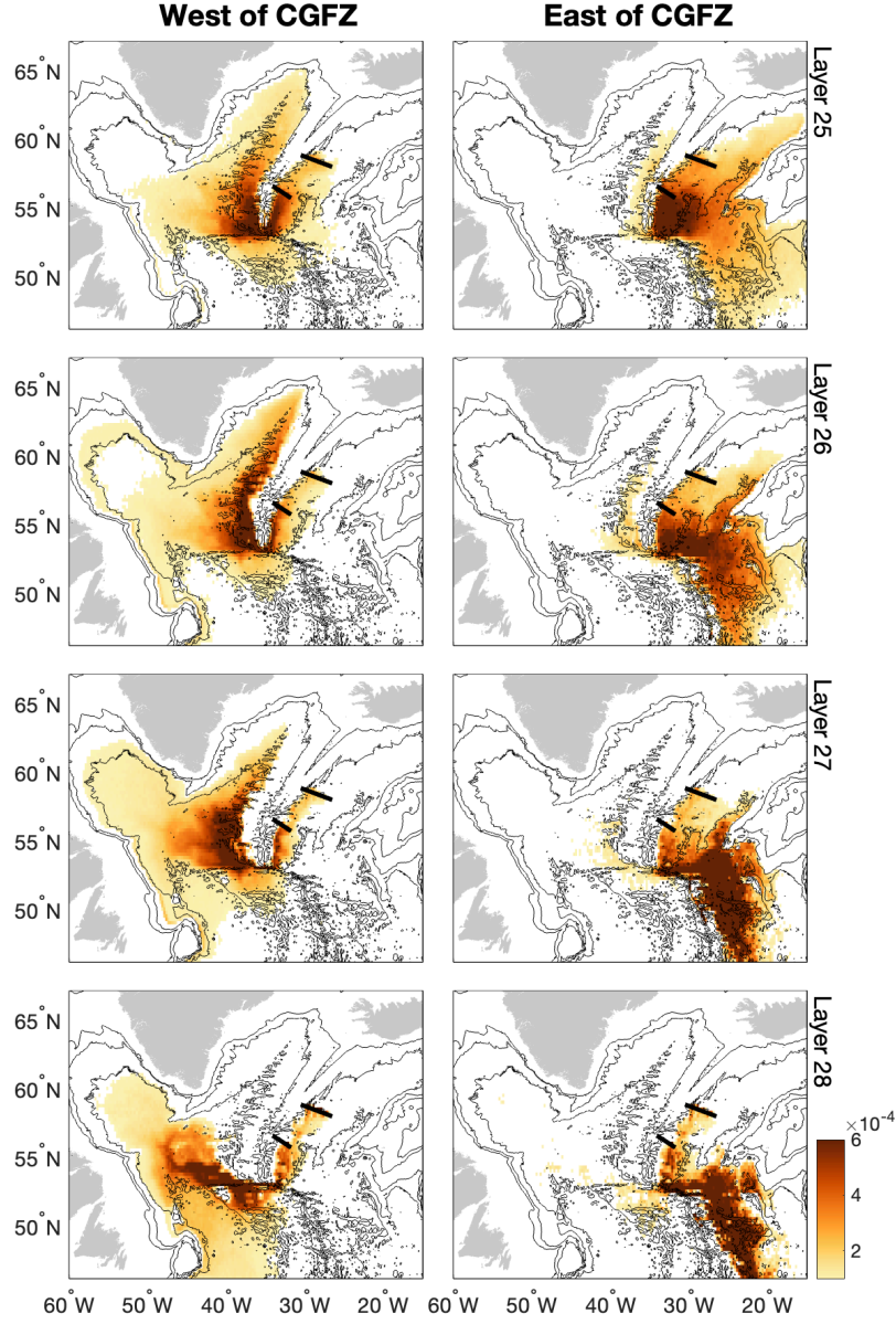
Figure 8: Probability distributions of 10-year simulated particle trajectories that traverse the Charlie Gibbs Fracture Zone after being initialized at two locations ( \sim 58^\circ\text{N} and \sim 56^\circ\text{N} ) along the eastern flank of the Reykjanes Ridge. The left column illustrates particles that propagate westward from the CGFZ and the right column illustrates particles that propagate eastward from the CGFZ. Each row represents the model layer particles were released within, from layer 25 in the top row to layer 28 in the bottom row. Black lines indicate particle release sites. Bathymetry is contoured every 1000 meters.
