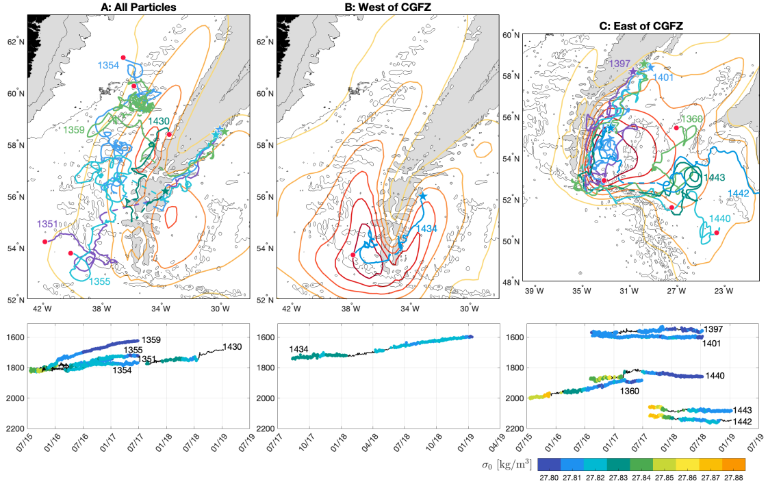
Figure 9: Top: RAFOS float trajectories overlaid on layer 25 particle distribution contour maps. Bottom: RAFOS along track pressure colored by isopycnal layer determined from the World Ocean Atlas. Only the RAFOS floats occupying the shallowest density ranges (on average 27.8 and 27.82 \text{ kg m}^{-3} ) are included. Sections of the float trajectories in dashed lines are times when coordinates could not be recovered and correspond to the time periods where pressure records are not colored. Stars indicate the initial float position and red circles indicate final float position. Trajectories and corresponding pressure records are labeled by RAFOS float serial number. From left to right (A to C) are particle distribution maps of all particles released within layer 25, particles that travel west from the CGFZ and particles that travel east from the CGFZ, respectively. Bathymetry shallower than 2000 meters is colored in gray and the 1000 , 2000 and 3000 meter isobaths are contoured on top.
