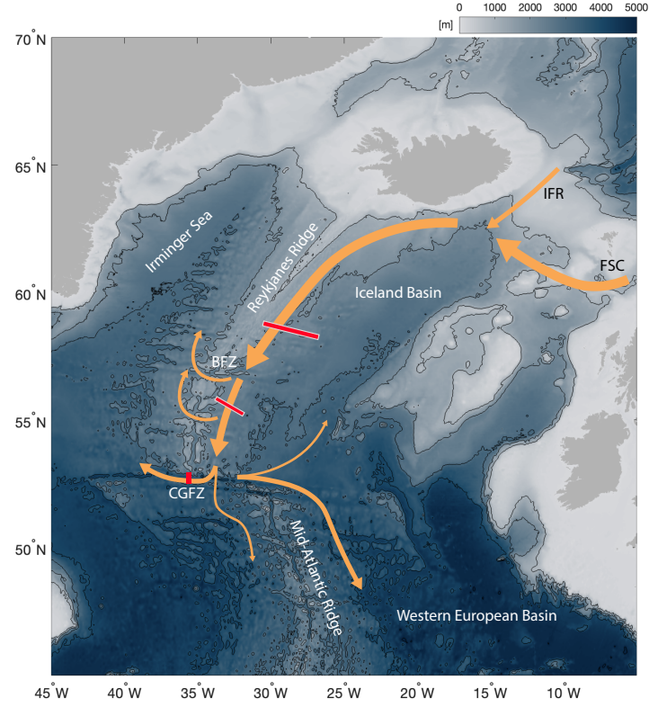
Figure 1: A schematic of Iceland-Scotland Overflow Water spreading pathways out of the Iceland Basin. Three solid red lines indicate the locations where RAFOS floats used in this study were released. Solid red lines outlined in white indicate the locations where simulated particles were released (co-located with float release locations east of the Reykjanes Ridge). Abbreviations are Charlie Gibbs Fracture Zone (CGFZ), the Bight Fracture Zone (BFZ), Iceland-Faroe Ridge (IFR) and Faroe-Shetland Channel (FSC).
