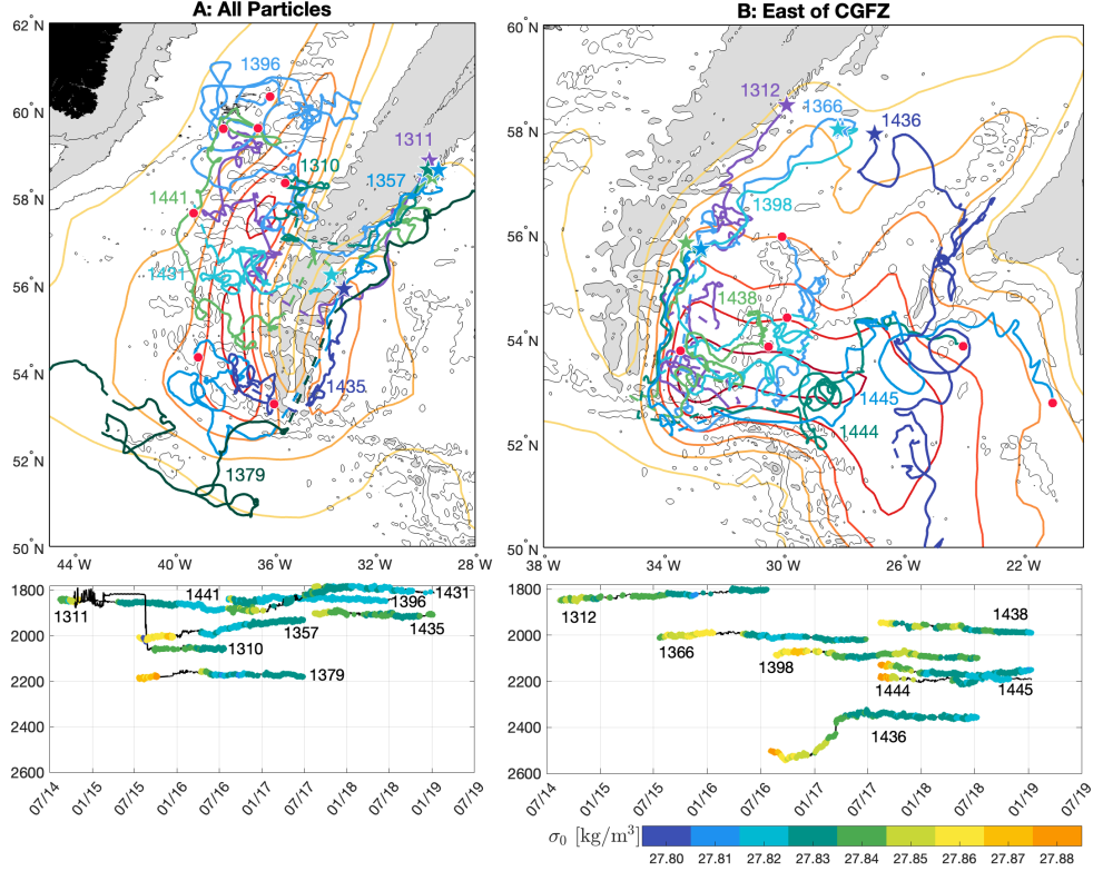
Figure 10: Same as Figure 9 except particle distribution maps are for layer 26 and RAFOS float trajectories occupy a density range of, approximately, between 27.82 - 27.84 \text{ kg m}^{-3} .
