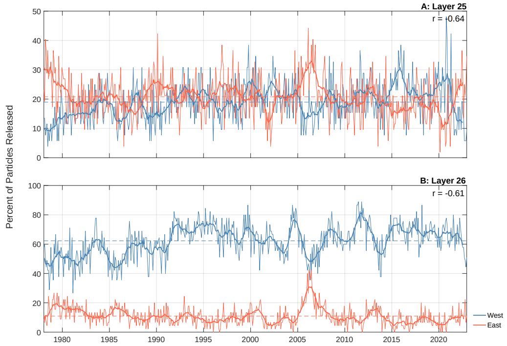
Figure 6: Percent of simulated particles released to successfully exit the Iceland Basin through the Charlie Gibbs Fracture Zone (western export, blue lines) vs. those that are deflected eastward (red lines) after entering the CGFZ in layer 25 (top) and layer 26 (bottom). Time series are smoothed using a 12-month boxcar moving mean filter and plotted on top of the monthly time series.
