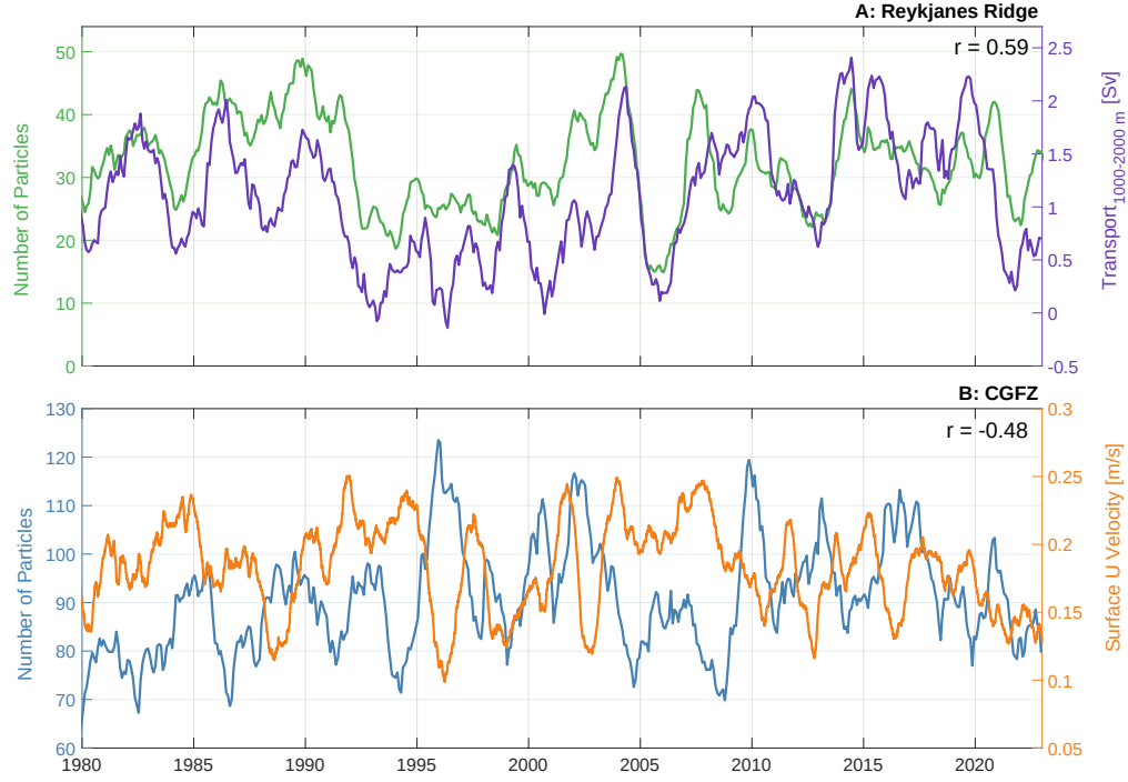
Figure 5: Controls on particle export over the Reykjanes Ridge (A) and through the CGFZ (B). A) Number of particles exported from the Iceland Basin to travel over the Reykjanes Ridge (green) compared transport across 53.80^{\circ}\text{N} between 1000 – 2000 meters depth. The number of particles only includes those from layer 25 & 26 and are binned monthly by their initial cross date over the Reykjanes Ridge gate. Transports are calculated from monthly HYCOM outputs. B) Number of particles that are deflected westward from the CGFZ (blue) vs. the zonal surface velocity averaged within the CGFZ (orange). The number of particles represents all layers collectively. Zonal velocities are calculated from daily HYCOM outputs. All time series are smoothed using a 12-month boxcar moving mean filter.
